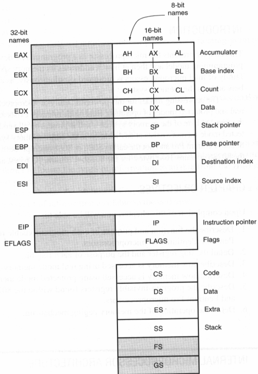
FIGURE 2-1 The programming model of the Intel 8086 through the Pentium Pro
