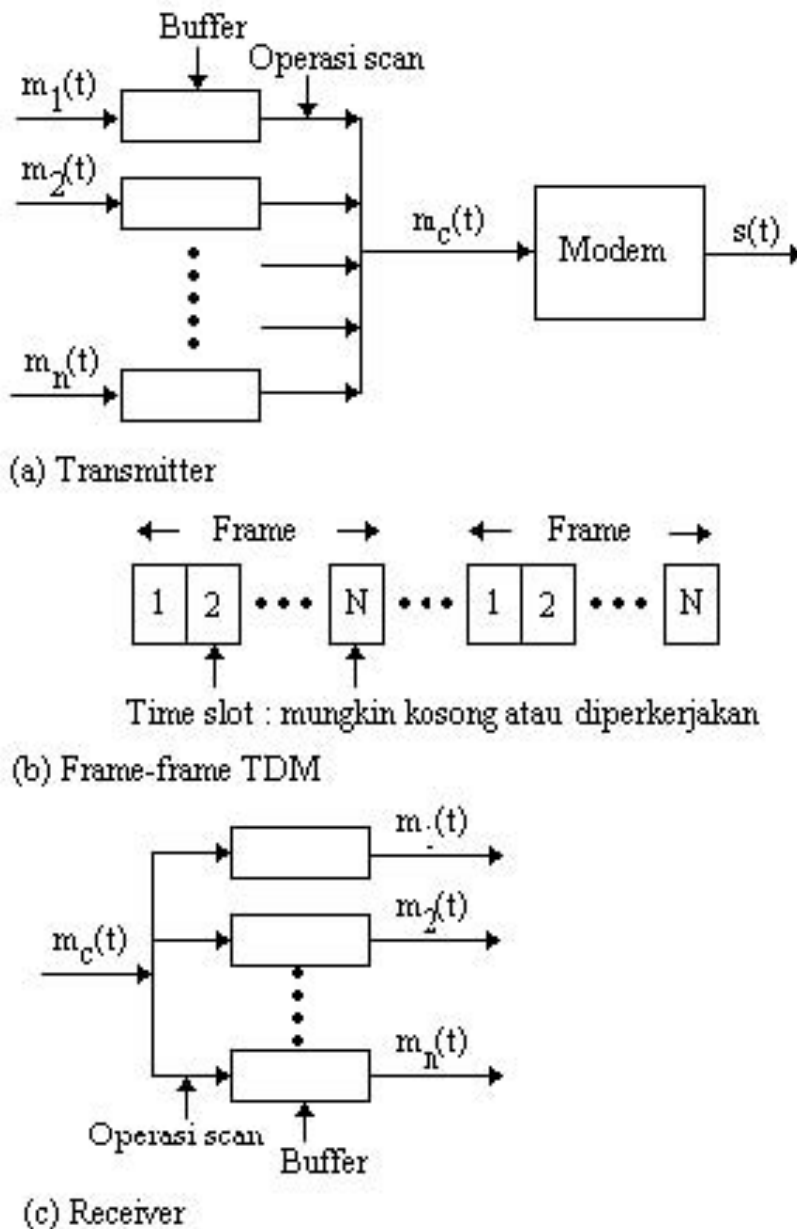
Gambar 6.7. Synchronous Time-Division Multiplexing
