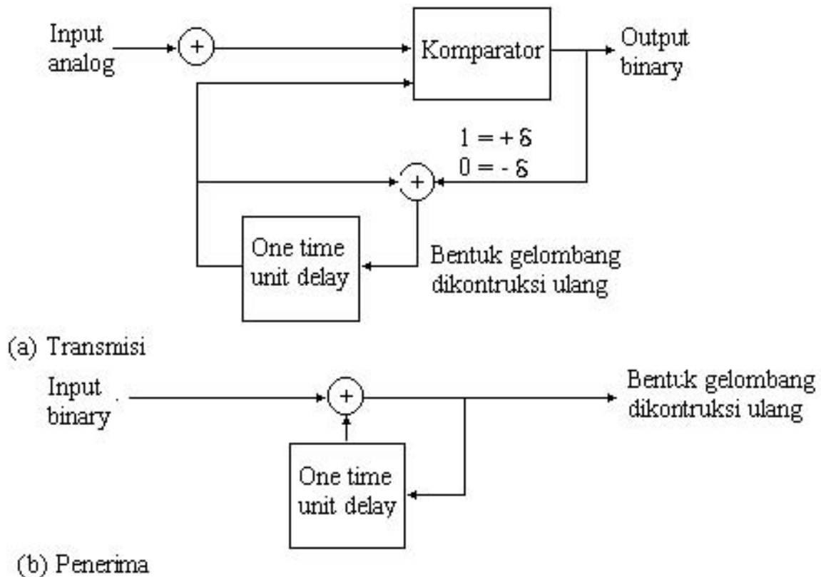
Gambar 3.16. Delta Modulation
