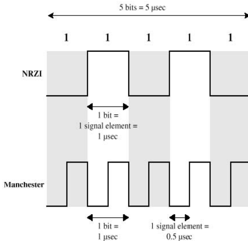
Gambar 3.2. Format Encoding Sinyal Digital
