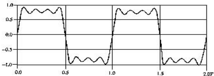
(b) \sin(2\pi f_1 t) + 1/3 \sin(2\pi(3f_1)t) + 1/5 \sin(2\pi(5f_1)t) + 1/7 \sin(2\pi(7f_1)t)
