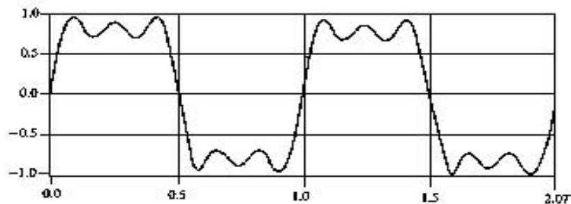
(a) \sin(2\pi f_1 t) + 1/3 \sin(2\pi(3f_1)t) + 1/5 \sin(2\pi(5f_1)t)
