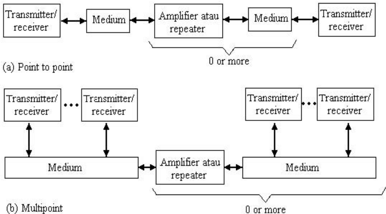
Gambar 2.1. Konfigurasi Guided transmission.
